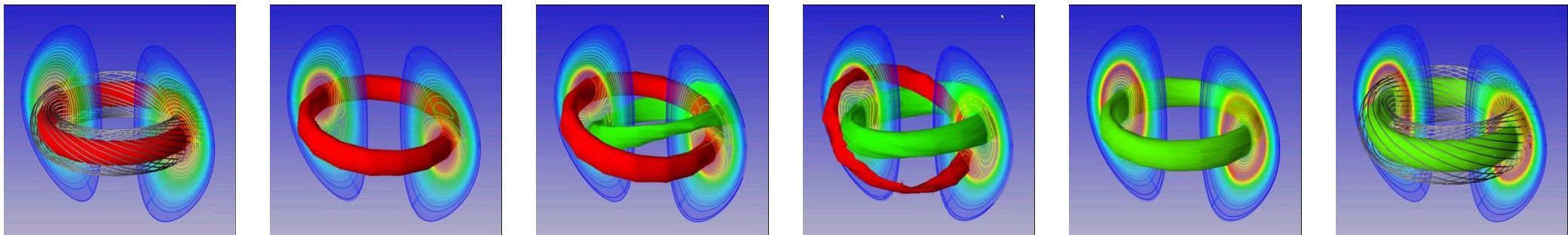
"Sawtooth" reconnection in a tokamak (NIMROD)
